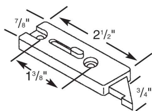
29750 - Tilt Latch -RH
