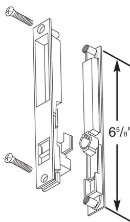
10170 - Without Key
