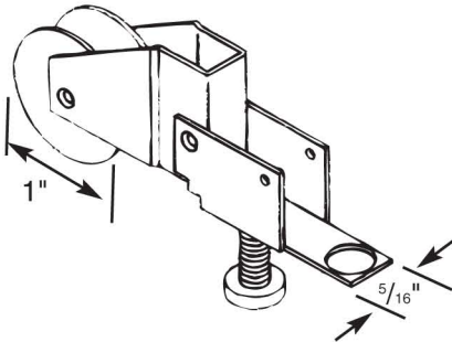
17290 - Nylon Roller
