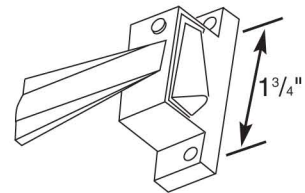
42281 Inside Latch
