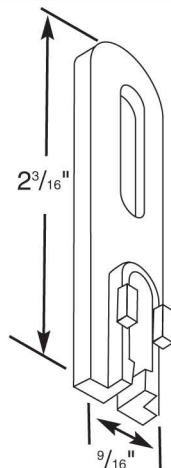
17530 - Screen Guides pair
