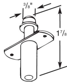
Spring Loaded Top Guide
