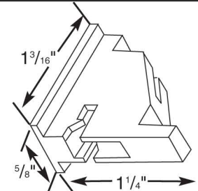
24670 - Balance Shoe
