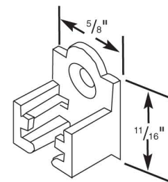
29280 - Lower Sash Clip
