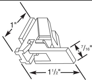
25560 - Balance Shoe
