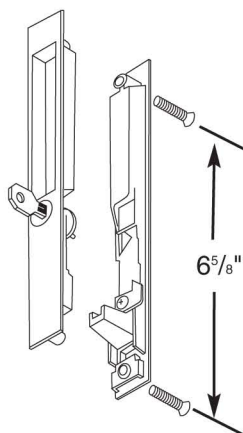
10270 - With Key
