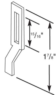
12040 - Screen Keeper
