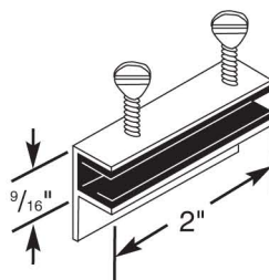
19110 Security Latch
