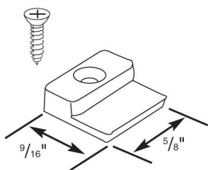
24250 -Face Guide with Screw
