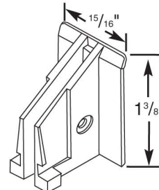
24660 - Balance Shoe
