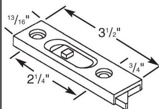
28204 - RH Tilt Latch
