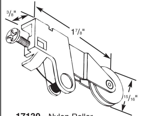
17130 - Nylon Roller
