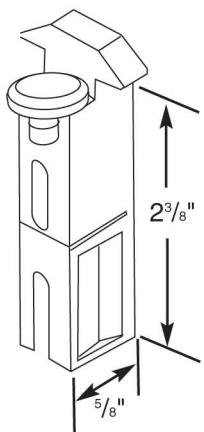
17240 - Nylon Roller pair
