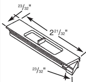
28206 - RH Tilt Latch -White
