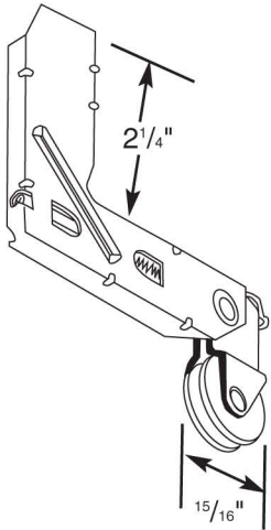
17080 - Nylon Roller 17081 - Steel Roller
