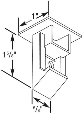
N24120 - Top Sash Guide
