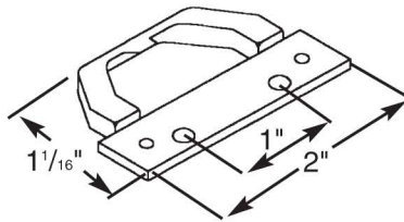
29622 - Keeper - White 29623 - Keeper - Black 29625 - Keeper - Beige
