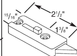
29880 - RH Tilt Latch - White
