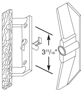
10020 - With Key 10030 - Without Key
