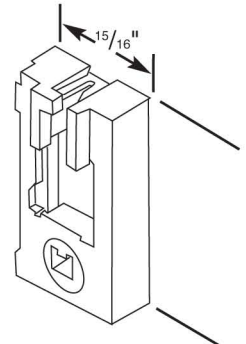
29400 - Pivot Shoe
