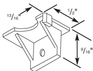
25930 pair - Top Sash Guide
