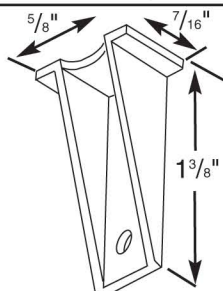
25830 - Top Sash Guide
