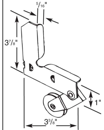
17082 - Nylon Roller 1 5/16" Diameter
