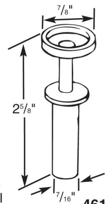
Top Guide Wheel
