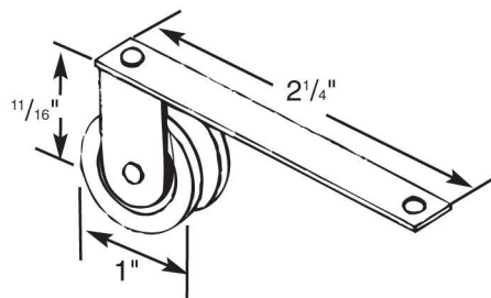
17120 - Nylon Roller
