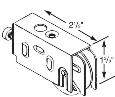
Wheel Diameter 1 1/2" 14450 14060 - 1 1/4" Wheel
