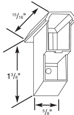
25640 - Top Sash Guide
