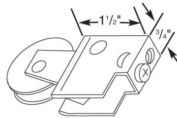
Wheel Diameter 1 1/2" 14040
