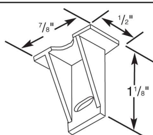
28600 - Top Sash Guide
