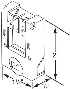
28210 - Pivot Shoe
