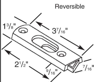
N29830 - Tilt Latch -White
