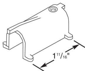
28520 - 1 11/16" Sash Stop 28521 - 1 1/16" Sash Stop
