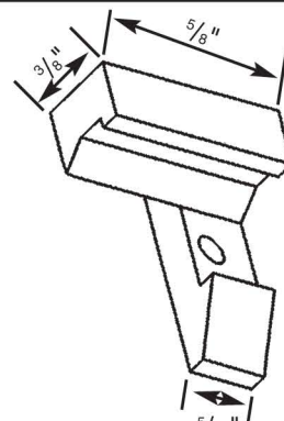
29661 - Top Sash Guide Pair
