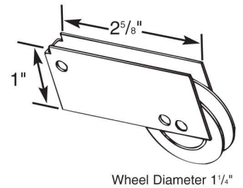
14431 - Steel Wheel 14430 - Plastic Wheel
