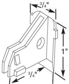
24370 - Balance Shoe
